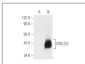
CRELD2 (C-6): sc-393980. Western blot analysis of CRELD2 expression in non-transfected: sc-117752 (A) and mouse CRELD2 transfected: sc-119455 (B) 293T whole cell lysates.
