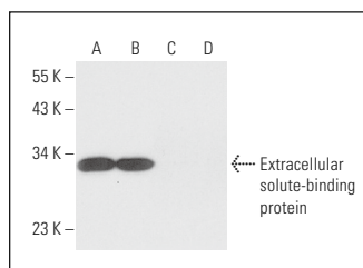
Extracellular solute-binding protein (E-11): sc-398029. Western blot analysis of Extracellular solute-binding protein expression in Streptococcus equi (virulent) (A), Streptococcus equi (avirulent) (B), Rhodococcus equi (C) and Escherichia coli (D) whole cell lysates. Note lack of reactivity with unrelated bacterial lysates in lanes C and D.
