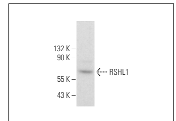
RSHL1 (C-4): sc-398329. Western blot analysis of RSHL1 expression in TT whole cell lysate.
