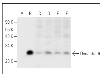
Dynactin 6 (F-9): sc-398647. Western blot analysis of Dynactin 6 expression in non-transfected 293T: sc-117752 (A), human Dynactin 6 transfected 293T: sc-113306 (B), HeLa (C), WI-38 (D), COLO 320DM (E) and T24 (F) whole cell lysates.
