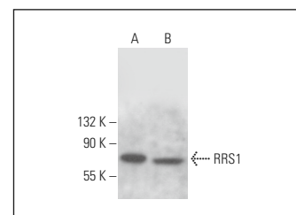
RRS1 (G-2): sc-398748. Western blot analysis of RRS1 expression in HL-60 nuclear extract (A) and 3T3-L1 whole cell lysate (B).
