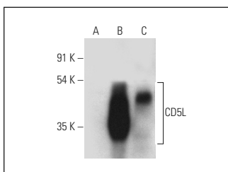
CD5L (F-1): sc-514283. Western blot analysis of CD5L expression in non-transfected 293T: sc-117752 (A) and human CD5L transfected 293T: sc-114208 (B) whole cell lysates and human spleen tissue extract (C).
