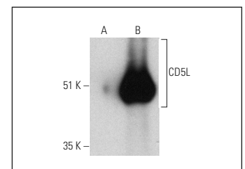
CD5L (F-1) HRP: sc-514283 HRP. Direct western blot analysis of CD5L expression in non-transfected: sc-117752 (A) and human CD5L transfected: sc-114208 (B) 293T whole cell lysates.
