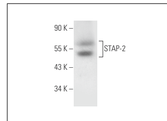
STAP-2 (H-10): sc-514716. Western blot analysis of STAP-2 expression in CSMLO whole cell lysate.
