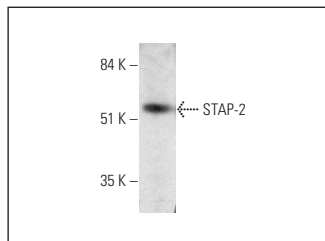
STAP-2 (H-10): sc-514716. Western blot analysis of STAP-2 expression in c4 whole cell lysate.
