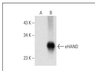
eHAND (E-6): sc-515047. Western blot analysis of eHAND expression in non-transfected: sc-117752 (A) and human eHAND transfected: sc-110104 (B) 293T whole cell lysates.
