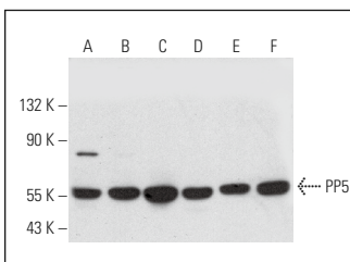
PP5 (G-6): sc-515257. Western blot analysis of PP5 expression in Hep G2 (A), A549 (B), Neuro-2A (C), EOC 20 (D), C6 (E) and KNRK (F) whole cell lysates.
