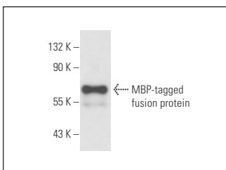
MBP-probe (R3.2): sc-53366. Western blot analysis of MBP-tagged fusion protein.
