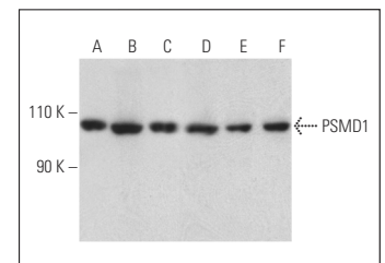
PSMD1 (C-7): sc-166038. Western blot analysis of PSMD1 expression in Hep G2 (A), K-562 (B), Jurkat (C), JAR (D), HeLa (E) and Sol8 (F) whole cell lysates. Detection reagent used: m-IgG 2b BP-HRP: sc-542741.
