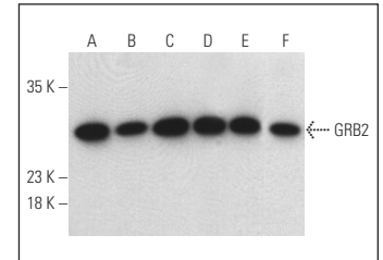
GRB2 (E-1): sc-17813. Western blot analysis of GRB2 expression in Jurkat (A), HEK293 (B), Ramos (C), HL-60 (D), MOLT-4 (E) and C6 (F) whole cell lysates. Detection reagent used: m-IgG 2b BP-HRP: sc-542741.
