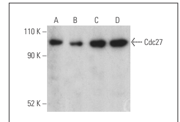
Cdc27 (AF3.1): sc-9972. Western blot analysis of Cdc27 expression in K-562 (A) and HEL 92.1.7 (B) whole cell lysates and A-431 (C) and Jurkat (D) nuclear extracts. Detection reagent used: m-IgG 2b BP-HRP: sc-542741.
