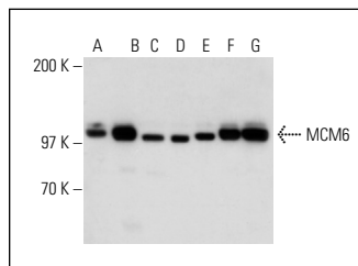
MCM6 (B-4): sc-55576. Western blot analysis of MCM6 expression in HeLa (A), ALL-SIL (B), MM-142 (C), NIH/3T3 (D), KNRK (E), K-562 (F) and Jurkat (G) whole cell lysates.
