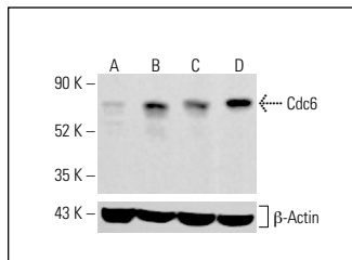
Cdc6 (O.T.17): sc-70826. Western blot analysis of Cdc6 expression in untreated (A) and chemically-treated (B, C, D) HeLa whole cell lysates. β-Actin (C4): sc-47778 used as loading control. Detection reagent used: m-IgG Fc BP-HRP: sc-525409.
