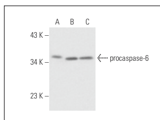
caspase-6 (7.1.65): sc-73539. Western blot analysis of procaspase-6 expression in PMA-treated Jurkat (A), staurosporine-treated Jurkat (B) and FAS-treated Jurkat (C) whole cell lysates.
