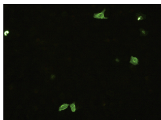
Influenza B NP (1D8/B1): sc-80483. Immunofluorescence staining of acetone-fixed, influenza B-infected Vero cells showing cytoplasmic and nuclear localization.
