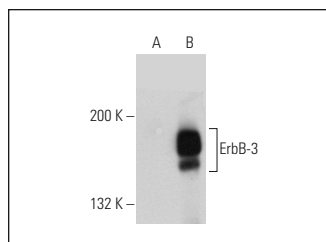
ErbB-3 (11A4): sc-81454. Western blot analysis of ErbB-3 expression in non-transfected: sc-117752 (A) and human ErbB-3 transfected: sc-111418 (B) 293T whole cell lysates.
