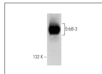
ErbB-3 (11A4): sc-81454. Western blot analysis of ErbB-3 expression in T-47D whole cell lysate.
