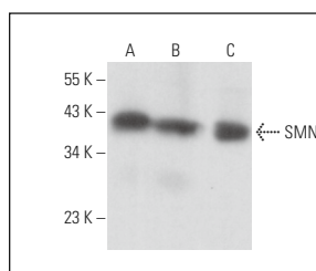
SMN (MANSMA1): sc-81555. Western blot analysis of SMN expression in K-562 (A), HEL 92.1.7 (B) and c4 (C) whole cell lysates.
