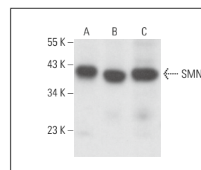
SMN (MANSMA1): sc-81555. Western blot analysis of SMN expression in 3T3-L1 (A) and BYDP (B) whole cell lysates and rat lymph node tissue extract (C).
