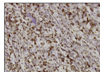
Rab 27a (E12A-1): sc-81914. Immunoperoxidase staining of formalin-fixed, paraffin-embedded human lymphoma tissue showing membrane and cytoplasmic localization.
