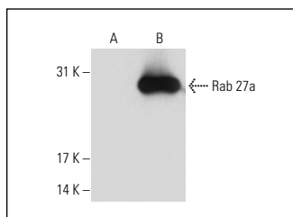
Rab 27a (E12A-1): sc-81914. Western blot analysis of Rab 27a expression in non-transfected: sc-117752 (A) and human Rab 27a transfected: sc-111961 (B) 293T whole cell lysates.
